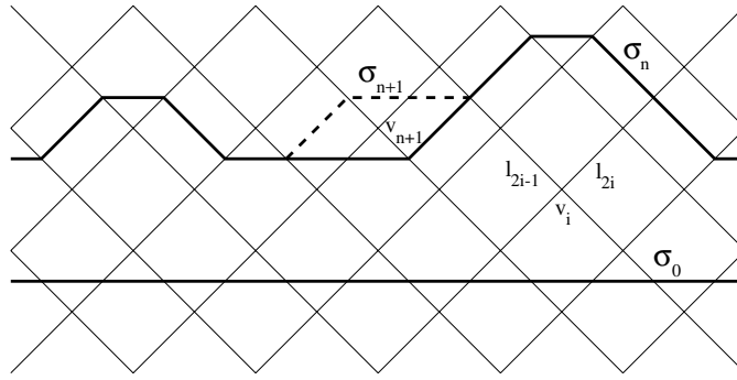
Figure 1. The light cone lattice. \sigma_0 is the initial surface and \sigma_n is a generic spacelike surface. The surface \sigma_{n+1} is shown after the vertex v_{n+1} is evolved over. A vertex v_i is shown with its two outgoing links, l_{2i-1} to the left and l_{2i} to the right.
